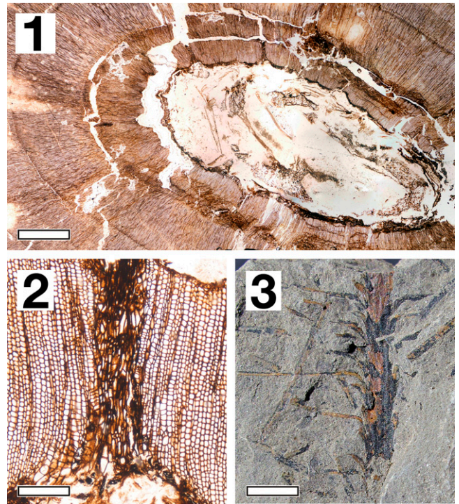
Fig. 1. Pennsylvanian coniferopsids like Giblingodendron (12) grew in central tropical Pangaea in and around cold and arid mountainous terrains. This putative dicranophyll was characterized by a dense pycnoxylic axis with small-diameter tracheids (1), a deciduous phenology as indicated by leaf traces abscised at the first ring boundary (2), and needle-like shoots, probably of Dicranophyllum type (3). These features are consistent with its being a frost-tolerant specialist. Frost selection of traits may have also conferred adaptation to aridity, paving the way for early conifers to dominate the hot Mesozoic Era that followed, as hypothesized by Matthaues et al. in PNAS (6). (Scale bars: 1, 5 mm; 2, 250 \mu m; 3, 5 mm.)
